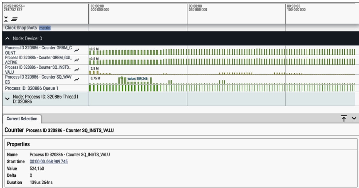
Fig. 2: Viewing kernel profiling output
