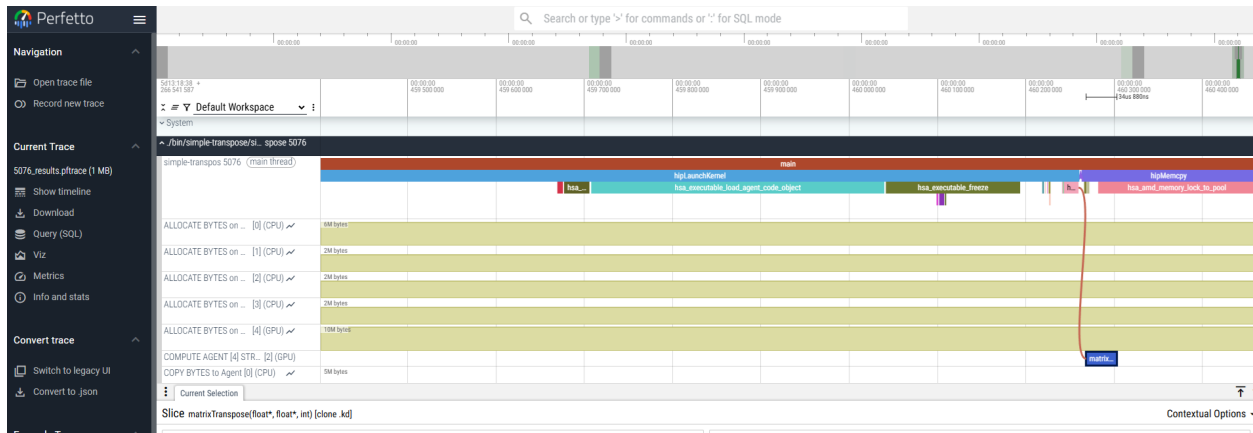
Figure 2: Visualization of ROCm flow data in Perfetto
